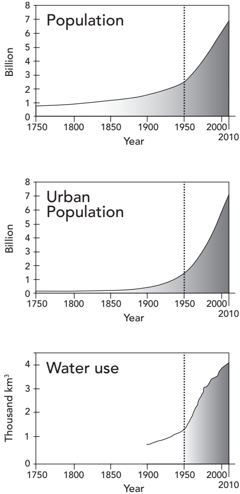
Figure 1. Trends from 1750 to 2010 in globally aggregated global and urban populations and of global water use. Water use includes agricultural, domestic and industrial uses
